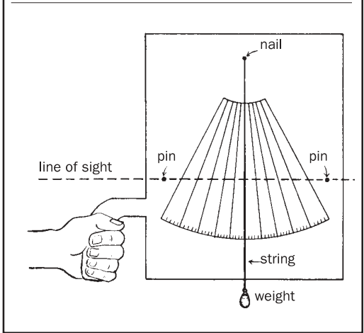
Figure 4. A slope finder is useful to determine slope.
