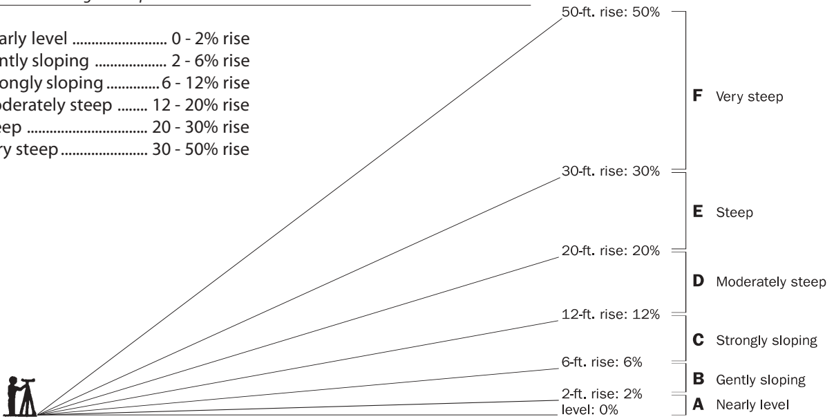
Figure 3. Percentage of slope.
